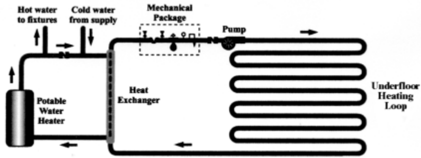
FIGURE 1—INDIRECT SYSTEM
