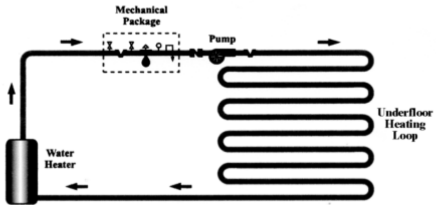
FIGURE 2—CLOSED SYSTEM
